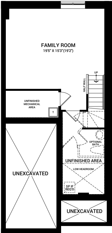
BASEMENT PLAN
